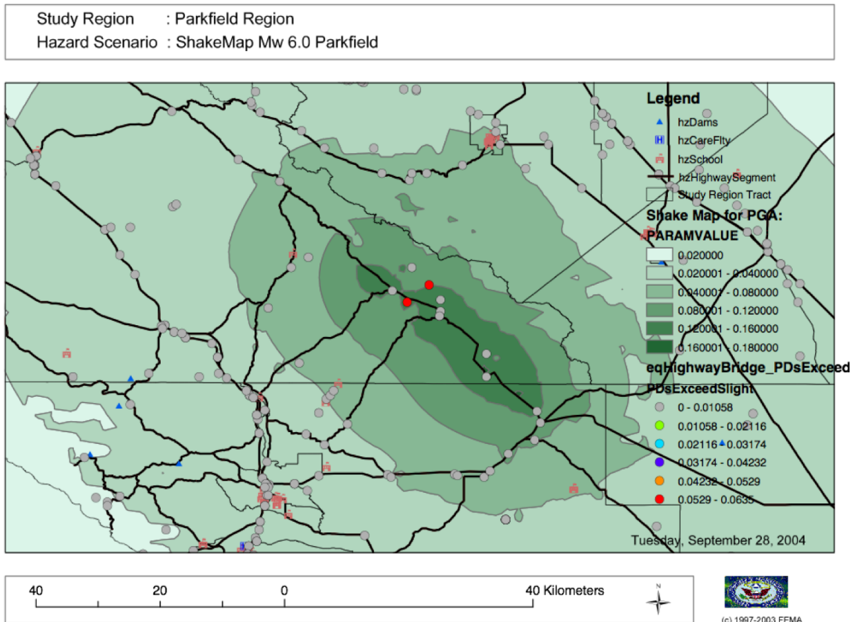
Fig. 1.39: 2004 M6.0 Parkfield, CA earthquake ShakeMap shapefiles (green polygons) and HAZUS estimated impact to selected infrastructure (circles) examined. Figure courtesy of D. Bausch, FEMA.
