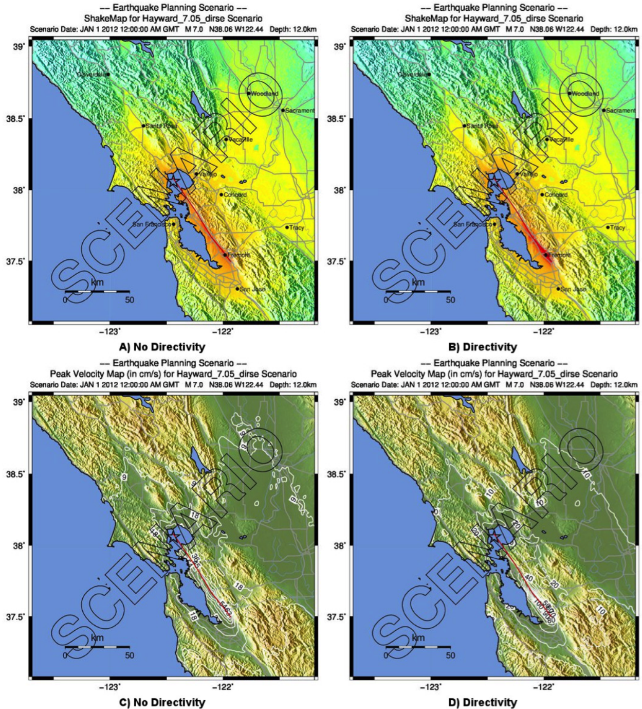
Fig. 1.33: ShakeMap scenario intensity (top) and peak velocity (bottom) maps for a M7.05 Hayward Fault, CA, earthquake: A) intensity; no directivity, B) intensity; directivity added, C) peak velocity; no directivity, and D) peak velocity; directivity added.
