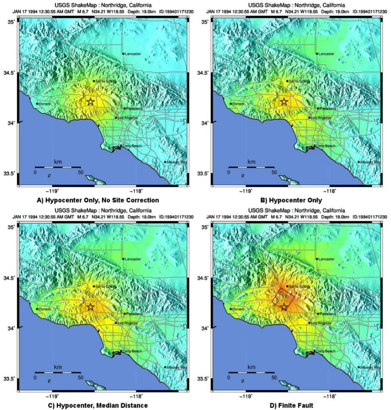
Fig. 1.10: ShakeMap intensity maps for the 1994 M6.7 Northridge, CA earthquake without strong motion or intensity data. A) Hypocenter only, without site amplification; B) Hypocenter, site amplification added; C) Hypocenter only, but with median distance correction added; and D) Finite fault (red rectangle) added.
