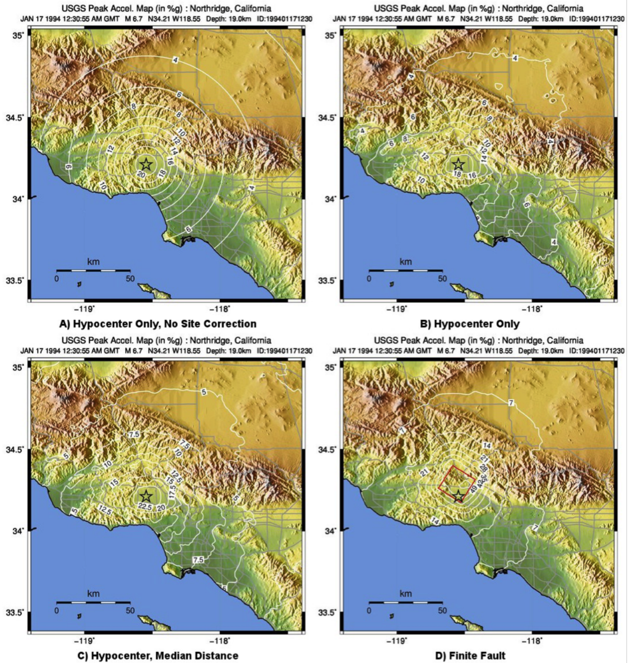
Fig. 1.9: ShakeMap peak ground acceleration maps for the 1994 M6.7 Northridge, CA earthquake without strong motion or intensity data. A) Hypocenter only, without site amplification; B) Hypocenter, site amplification added; C) Hypocenter only, but with median distance correction added; and D) Finite fault (red rectangle) added.
