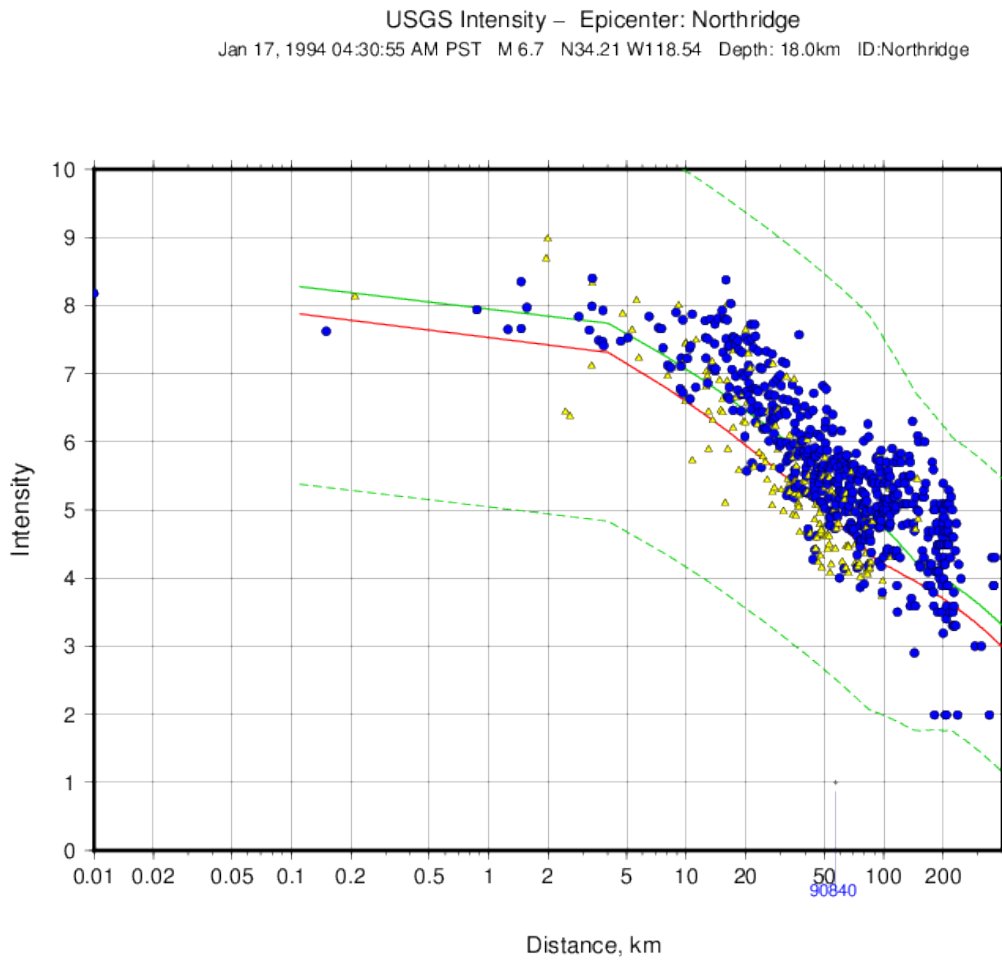
Fig. 1.27: Plot showing the 1994 M6.7 Northridge, CA earthquake MMI data (seismic stations are yellow triangles; DYFI observations are blue circles) plotted with the unbiased (red line) and biased (green line) IPE. The dashed green lines show the biased IPE \pm 3 standard deviations.
