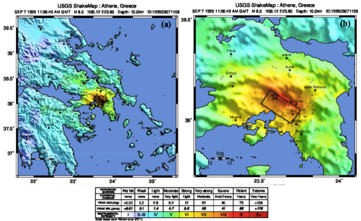
Fig. 1.31: Example of the macroseismic intensity ShakeMaps for one ShakeMap Atlas event: the 1999 M6.0 Athens, Greece earthquake. (A) overview map; and (B) zoomed map. The black rectangle delineates the surface projection of the finite fault (a normal fault dipping southwest). Circles represent native MMI data; triangles show PGM data converted to MMI values via the Worden et al. (2012) GMICE, the choice of which automatically redefines the legend scale. After Garcia et al. (2012a) .
