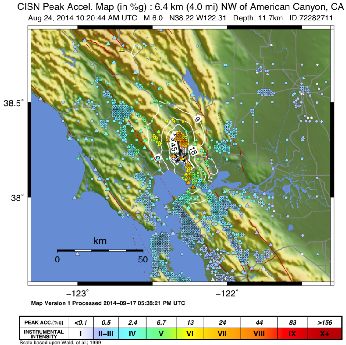
Fig. 1.5: Peak acceleration ShakeMap from the Aug. 24, 2014, M6.0 American Canyon (Napa Valley), California earthquake. Strong motion data (triangles) and intensity data (circles) are color-coded according to their intensity value, either as observed (for macroseismic data) or as converted by Wald et al. (1999b) as shown in the legend. The north-south black line indicates the fault location, which nucleated near the epicenter (red star). Note: Map Version Number reflects separate offline processing for this Manual.
