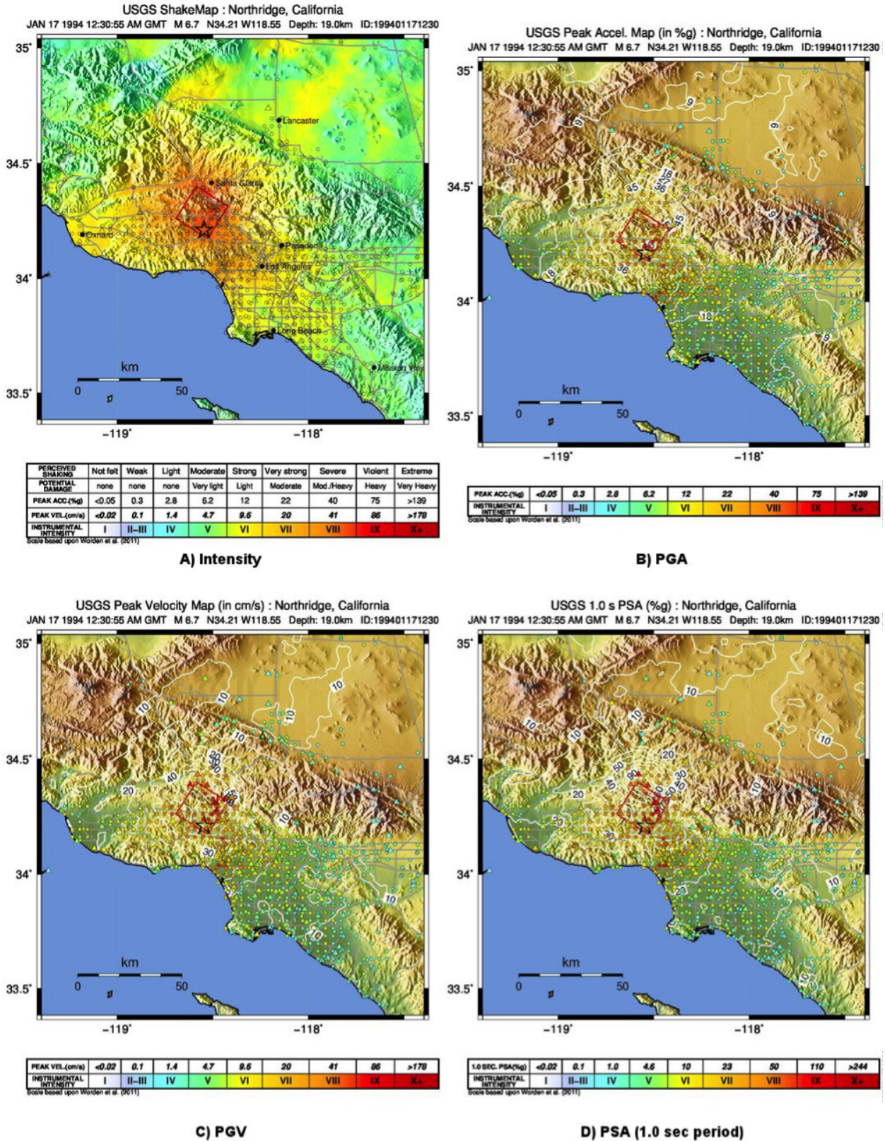
Fig. 1.18: ShakeMap for the 1994 M6.7 Northridge, CA earthquake with a finite fault (red rectangle), strong motion data (triangles) and intensity data (circles). Stations and macroseismic data are color coded according to their intensity value, either as observed (for macroseismic data) or as converted by Worden et al. (2011) and indicated by the scales shown. Note: Macroseismic data do not change colors from map to map, but seismic stations do, since the estimated intensity conversion depends on which parameter is used.
