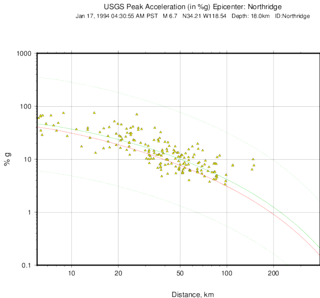
Fig. 1.11: Plot of Northridge earthquake PGAs as a function of distance. The triangles show recorded ground motions; the red line shows the unbiased Boore and Atkinson (2008) (BA08) GMPE; the dark green lines show BA08 following the bias correction described in the text; the faint green lines show the bias-adjusted GMPE +/- three standard deviations.
