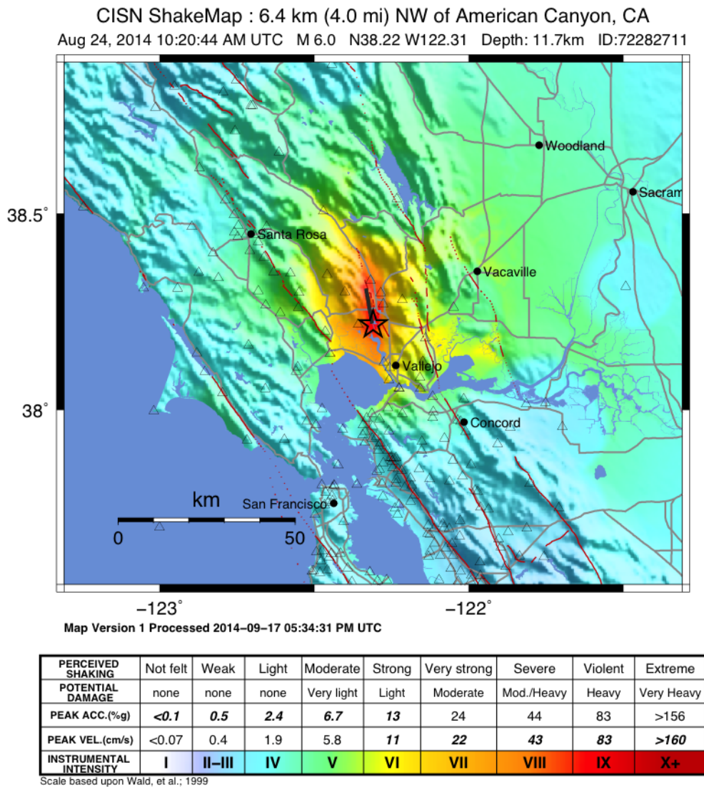
Fig. 1.20: Intensity ShakeMap from the 2014 M6.0 American Canyon (Napa Valley), CA earthquake. Strong-motion data (triangles) and intensity data (circles) default to “see-through” mode for the intensity map. The north-south black line indicates the fault location, and the epicenter is a red star. The intensity color-coding either as observed (for macroseismic data) or as converted is derived from the conversion equations of Wald et al. (1999b) as shown in the legend. Note: Map Version Number reflects separate offline processing for this Manual.
