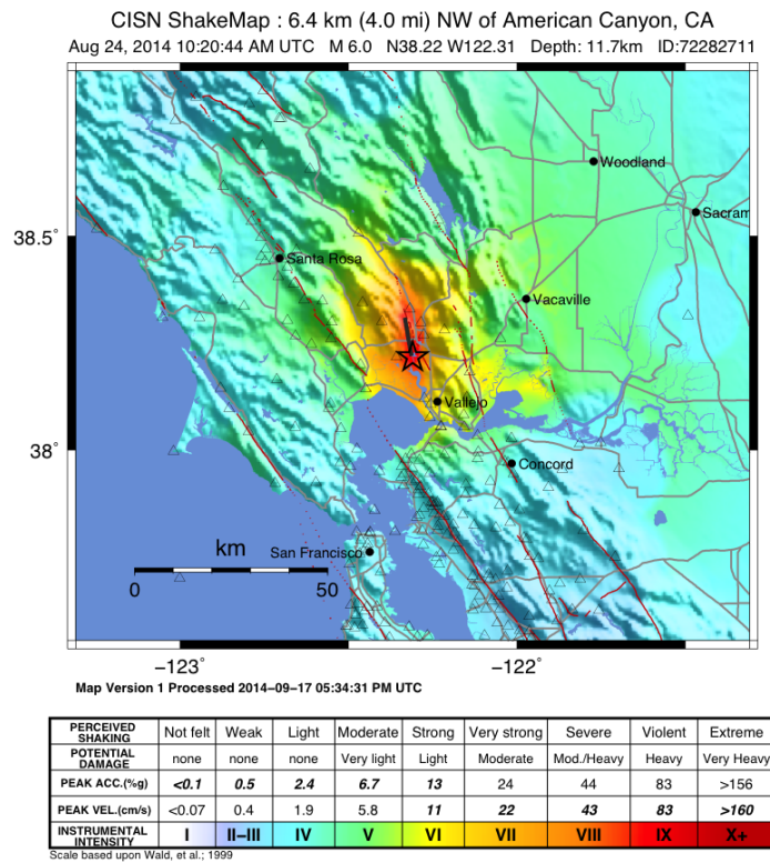
Fig. 1.1: 2014 M6.0 Napa, CA, earthquake intensity ShakeMap.
