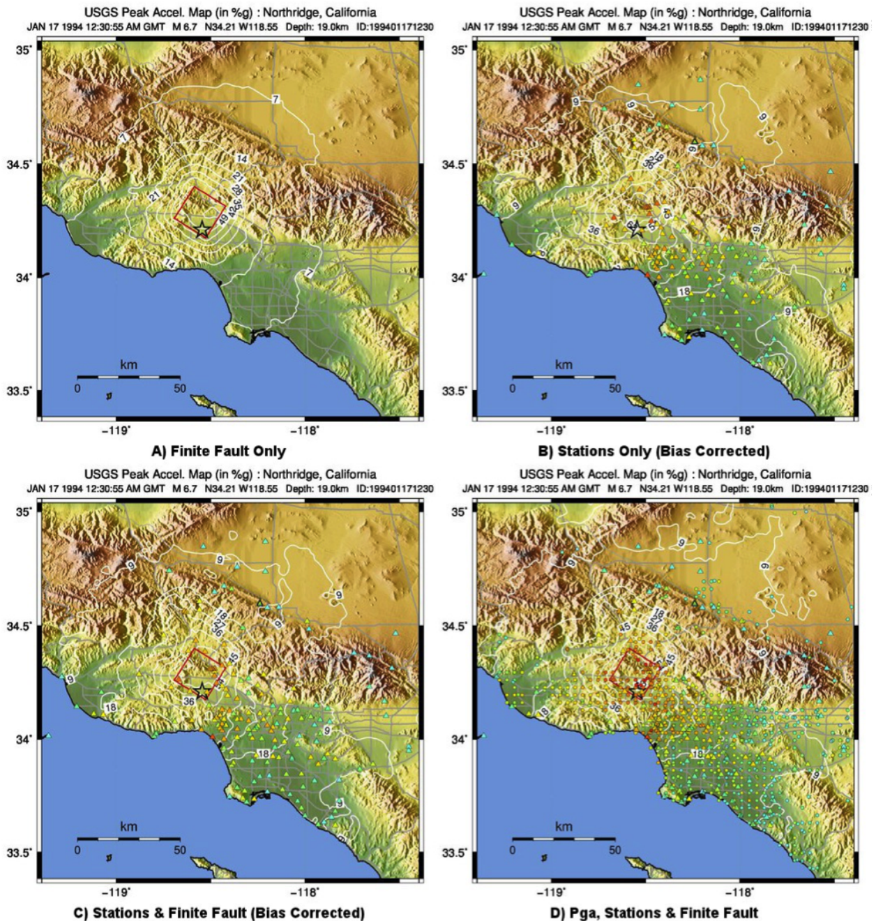
Fig. 1.13: PGA ShakeMaps for the Northridge earthquake, showing effects of adding strong motion and intensity data. A) Finite fault only (red rectangle), no data; B) Strong motion stations (triangles) only; C) Finite Fault and strong motion stations (triangles); D) Finite Fault strong motion stations (triangles) and macroseismic data (circles). Notes: Stations and macroseismic observations are color-coded to their equivalent intensity using Worden et al. (2012) .
