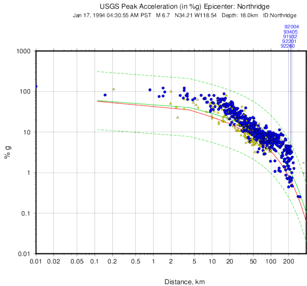
Fig. 1.28: Plot showing the 1994 M6.7 Northridge, CA earthquake PGA data (seismic stations are yellow triangles; DYFI observations are blue circles) plotted with the unbiased (red line) and biased (green line) GMPE. The dashed green lines show the biased GMPE \pm 3 standard deviations.
