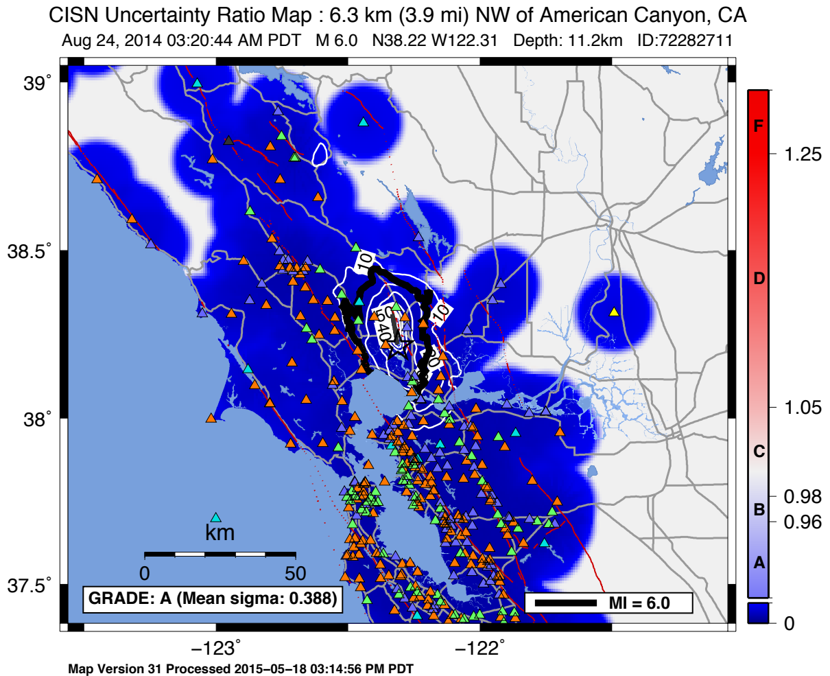
Fig. 1.26: ShakeMap uncertainty map for the 2014 M6.0 American Canyon, CA earthquake. Color-coded legend shows uncertainty ratio, where “1.0” indicates 1.0 times the GMPE’s sigma. The average uncertainty is computed by averaging uncertainty at grid points that lie within the MMI-VI contour (bold contour line). For more details, see Wald et al. (2008) , Worden et al. (2010) , and the Technical Guide .
