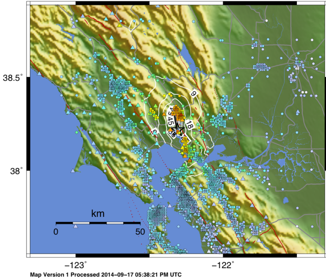
CISN Peak Accel. Map (in %g) : 6.4 km (4.0 mi) NW of American Canyon, CA Aug 24, 2014 10:20:44 AM UTC M 6.0 N38.22 W122.31 Depth: 11.7km ID:72282711
