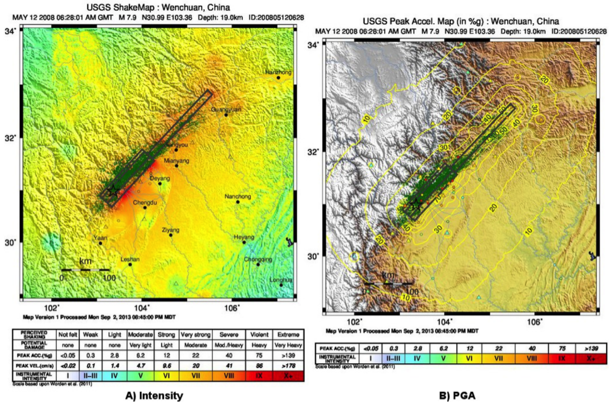
Fig. 1.32: Example of the ShakeMaps for the 2008 M 7.9 Wenchuan, China earthquake for (A) Intensity and (B) PGA. Green polygons show areas of landsliding mapped out by Dai et al. (2010) . Black rectangles delineate the surface projection of the different fault segments involved in the rupture. Triangles indicate native strong motion stations; circles represent MMI data converted to GM values via a GMICE (here Worden et al., (2012) , the choice of which automatically redefines the legend scale.
