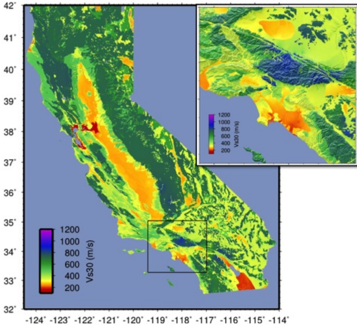
Fig. 1.8: Revised California Vs30 Map ( Thompson et al., 2014 ). This map combines geology, topographic slope, and constraints of map values near Vs30 observations using kriging-with-a-trend. Inset shows Los Angeles region, with Los Angeles Basin indicating low Vs30 velocities.
