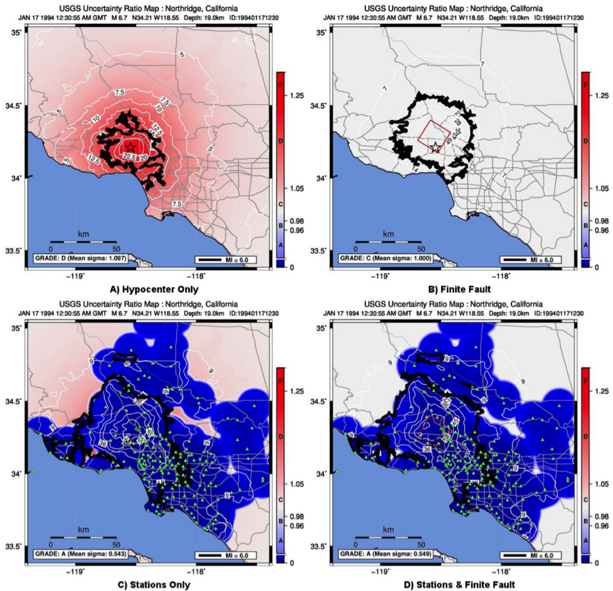
Fig. 1.16: ShakeMap uncertainty maps for the Northridge earthquake showing effect of adding a finite fault and strong motion data. Color-coded legend shows uncertainty ratio, where ‘1.0’ indicates 1.0 times the GMPE’s sigma. A) Hypocenter (black star) only; B) Finite fault (red rectangle) added but no data (mean uncertainty is 1.00 at all locations since the site-to-source distance is constrained); C) Hypocenter and strong motion stations (triangles) only (adding stations reduces overall uncertainty); and D) Finite fault and strong motion stations. Note: Average uncertainty is computed by averaging uncertainty at grids that lie within the MMI = VI contour (bold contour line), so panel (D) is marginally higher than (C) despite added constraint (fault model). For more details see Wald et al. (2008) and Worden et al. (2010) .
