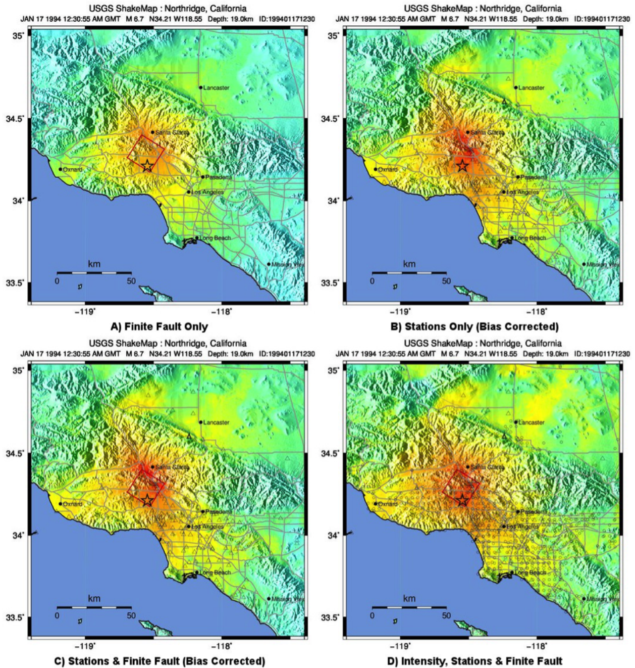
Fig. 1.14: Intensity ShakeMaps for the Northridge earthquake, showing effects of adding strong motion and intensity data. A) Finite fault only (red rectangle), no data; B) Strong motion stations (triangles) only; C) Finite Fault and strong motion stations (triangles); D) Finite Fault strong motion stations (triangles) and macroseismic data (circles). Notes: (D) is the best possible constrained representation for this earthquake. The finite fault model without data (A) is not bias-corrected; for the Northridge earthquake, the inter-event biases are positive, indicating higher than average ground shaking for M6.7; thus, the unbiased map (A) tends to under-predict shaking shown in the data-rich, best-constrained map (D).
